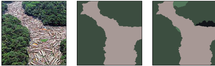
FIGURE 12. Unsupervised color image classification with L^1 norm, \alpha = 5.10^{-3}\sqrt{n} : original image (left, 231 \times 221 pixels), obtained image with 2 labels (middle), obtained image with 5 labels (right).
