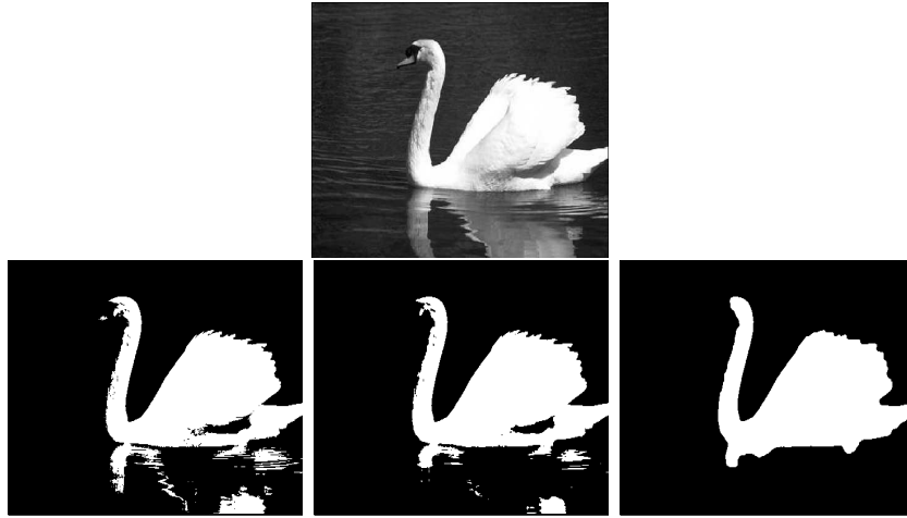
FIGURE 4. First row: original image ( 320 \times 480 pixels). Second row, from left to right: initialization ( \varepsilon = \infty ), and obtained solutions for \varepsilon = \varepsilon_{max}/16 and \varepsilon = \varepsilon_{min} , respectively (with \alpha = 9.10^{-3}\sqrt{n} ).
