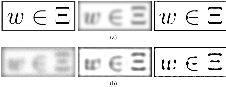
FIGURE 16. Deblurring of the text “ w \in \Xi ”. 16(a) Original image (left, 245 \times 600 pixels), blurred image (middle), reconstructed image for \alpha = 2.10^{-5}\sqrt{n} (right). 16(b) blurred image with noise (left), its restoration with \alpha = 2.10^{-5}\sqrt{n} for \varepsilon = 1.99 (middle) and for \varepsilon = \varepsilon_{min} (right).
