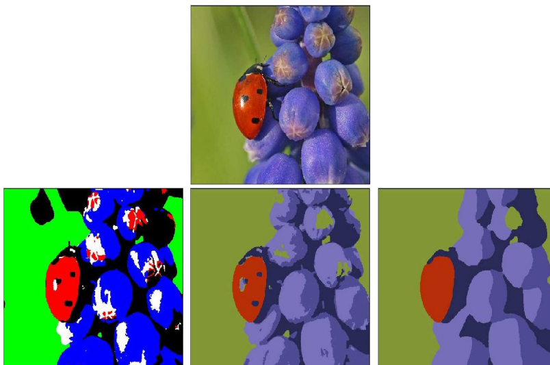
FIGURE 1. Color image classification. First row: original image ( 611 \times 471 pixels). Second row, from left to right: supervised solution for \alpha = 5 \cdot 10^{-4} \sqrt{n} ( n is the number of pixels), unsupervised solution for \alpha = 5 \cdot 10^{-4} \sqrt{n} and \alpha = 10^{-2} \sqrt{n} , respectively. TV-model with H = L^1 , A = I and 5 labels.
