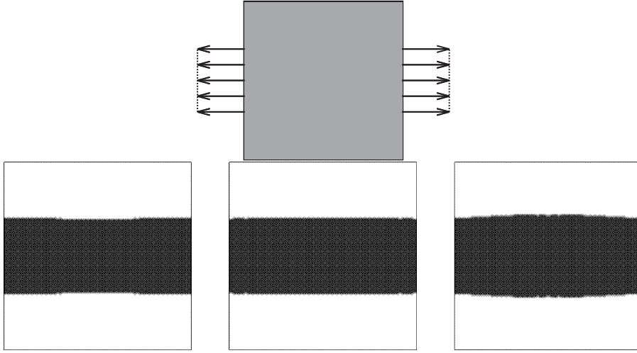
Fig. 4 Bar: boundary conditions and obtained domains for (\alpha, \beta) = (0, 1) , (\alpha, \beta) = (1, 0.2) and (\alpha, \beta) = (10, 0.2) , respectively.
