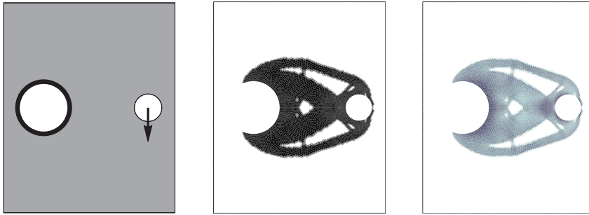
Fig. 5 Michell's structure: boundary conditions and unconstrained solution with the corresponding Von Mises stress distribution.
