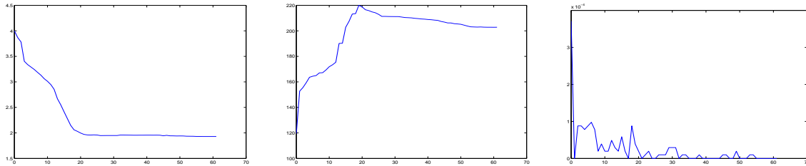
Fig. 9 L-beam with \bar{\sigma}_M = 30 : convergence history for the area, the compliance and the area of the region in which the constraint is violated (from left to right).
