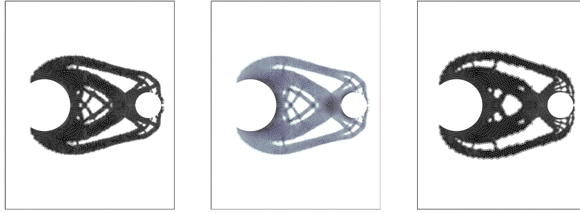
Fig. 6 Michell's structure: optimal domain for \alpha = 100 (left) and Von Mises stress distribution, optimal domain for \alpha = 500 (right).
