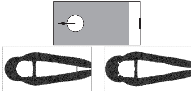
Fig. 7 Eyebar: boundary conditions and obtained domains for \alpha = 0 and \alpha = 500 .
