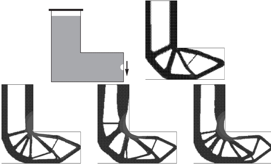
Fig. 8 L-beam: boundary conditions and obtained design in the unconstrained case (top), obtained designs with the penalization for \bar{\sigma}_M = 40 , \bar{\sigma}_M = 30 and \bar{\sigma}_M = 25 (bottom, from left to right).
